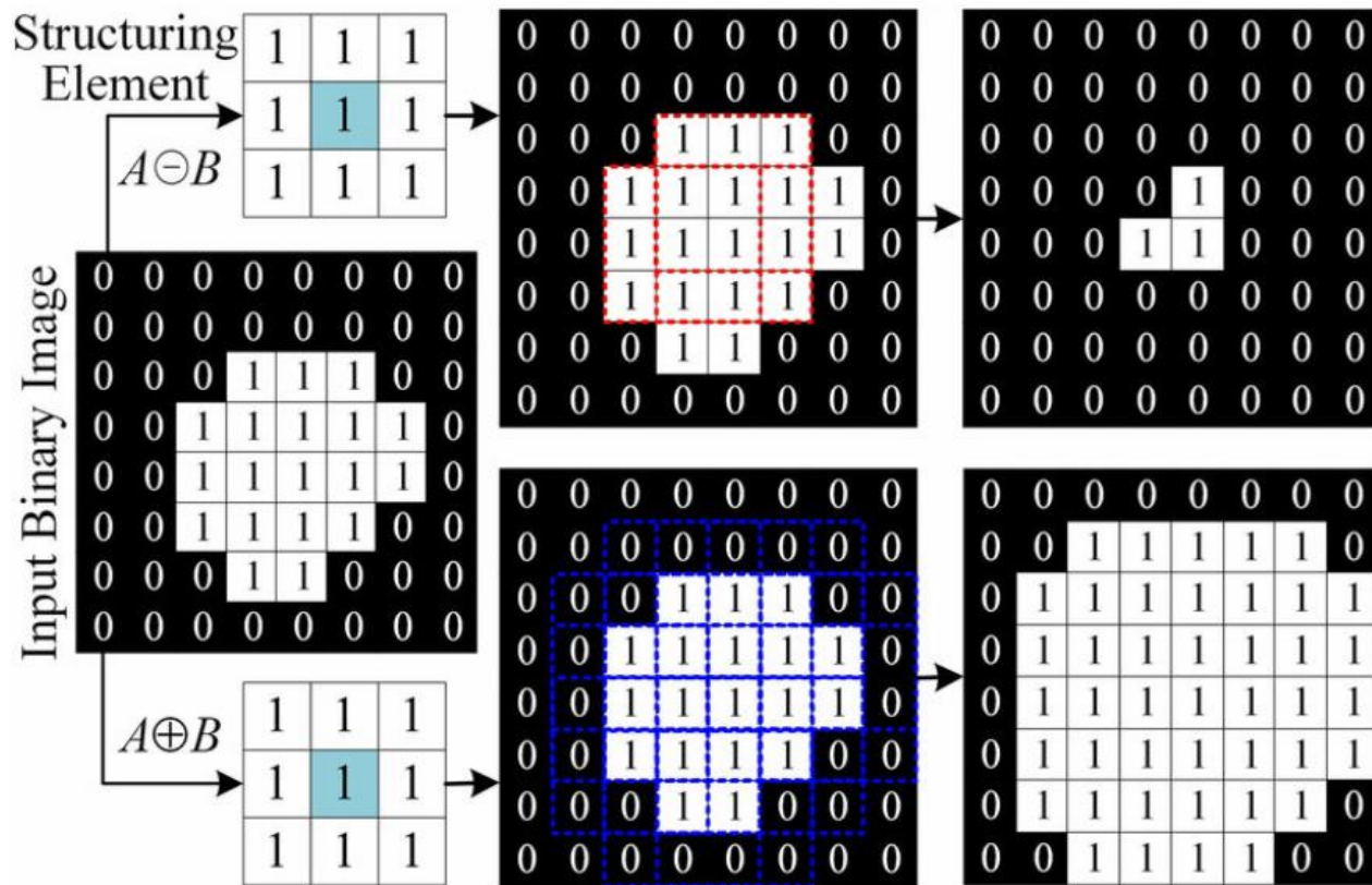
Example of erosion and dilation operation by a 3 \times 3 structuring elements.
