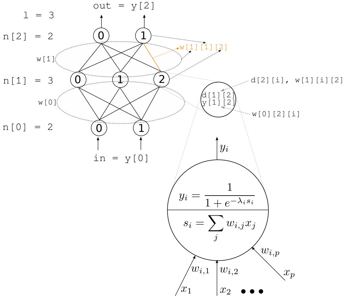
Figure 1: Neural Network Model
